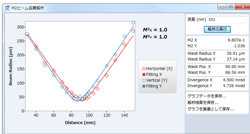
M 2 measurement example of commercially available green laser pointer
