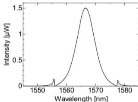
(Op/cal spectrum)
